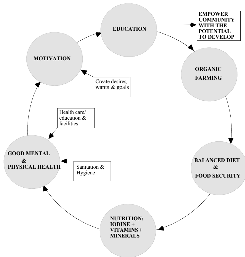
Fig. 2 Goals Diagram
